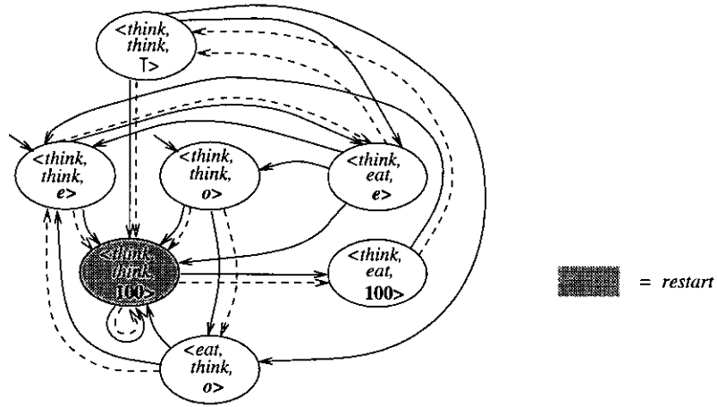
Figure 4: The mixed abstract model for the modified program.
