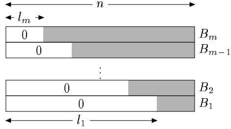
FIGURE 2. The pattern of leading zeros in the basis vectors B_1, B_2, \dots, B_m .
