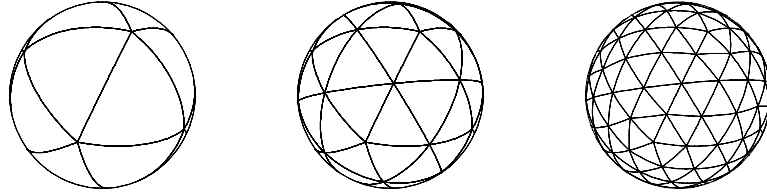
Figure 1 The geodesic sphere construction starting with the icosahedron on the left (subdivision level 0) and the next 2 subdivision levels. Successive levels are generated cutting each triangle into four children. This is accomplished by adding vertices at the midpoint of edges and connecting them with geodesics.
